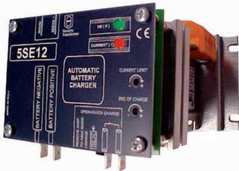
RAL5SE12 (5A - 12VDC) RAL5SE24 (5A - 24VDC)
