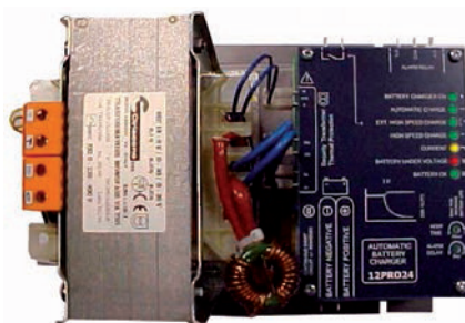
RAL12PRO24 (12A - 24VDC)
